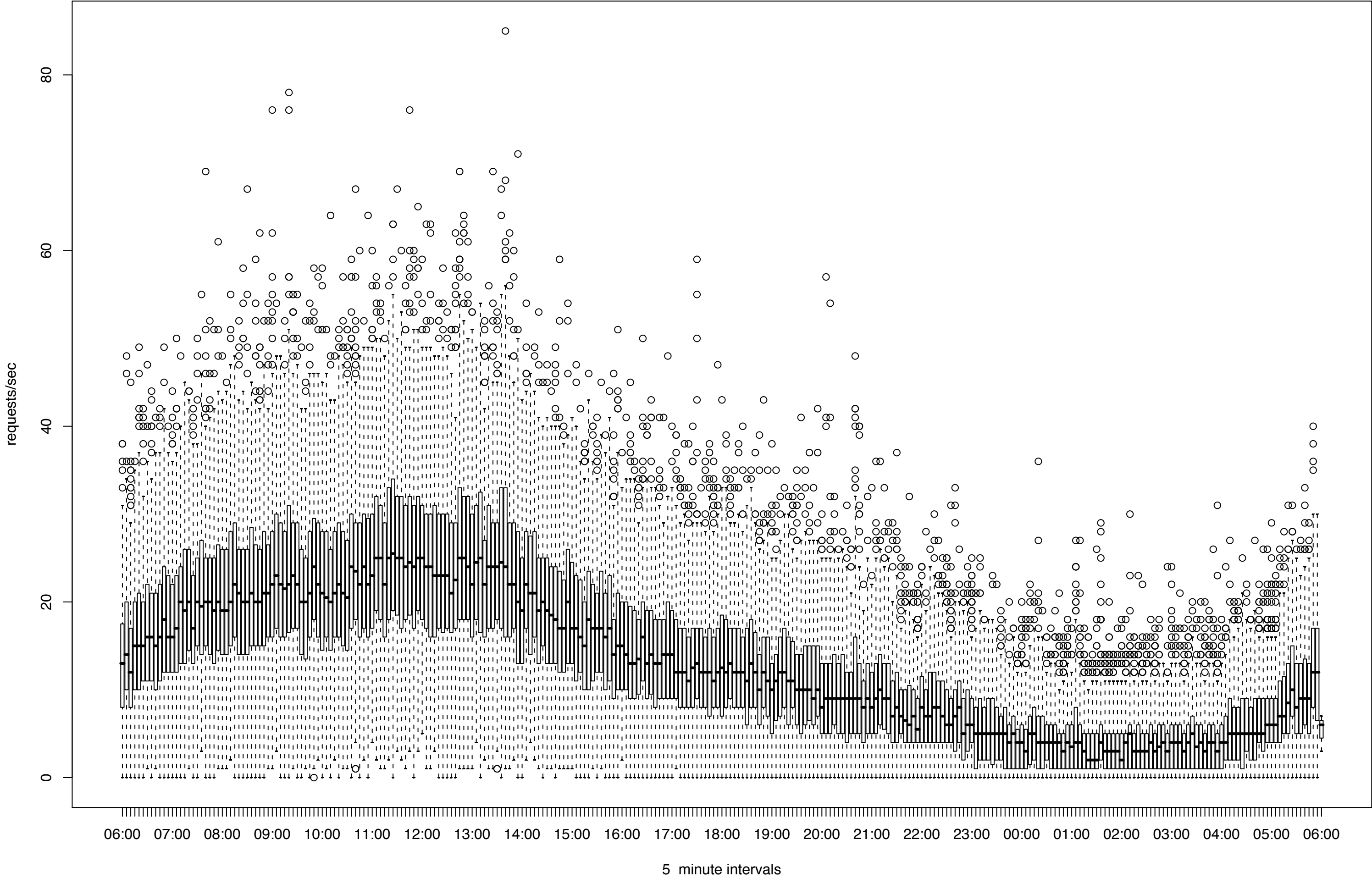
Requests per Second During Each Time Interval
